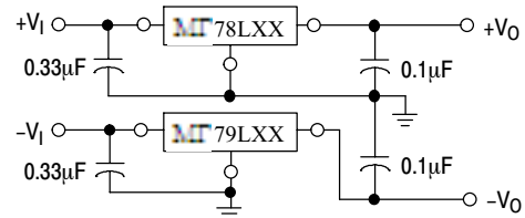
Figure 10. Positive and Negative Regulator
